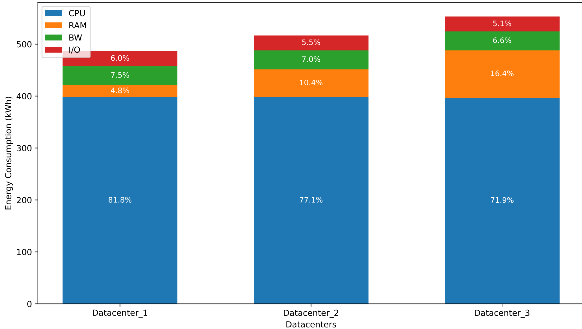
Optimized RAM: Power Consumption per Datacenter (Stacked by Component)
